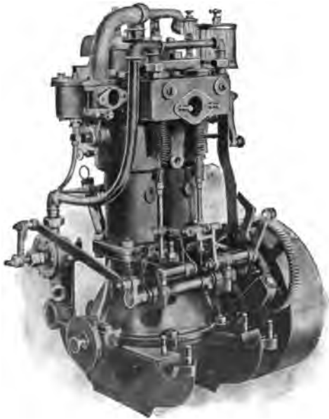
FIG. 378.—Double-vertical Cylinder Motor, used on the wagons manufactured by the American Daimler Co.
